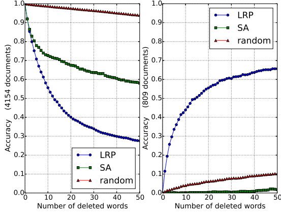
Figure 1: Word deletion on initially correct (left) and false (right) classified test documents, using either LRP or SA. The target class is the true document class, words are deleted in decreasing (left) and increasing (right) order of their relevance. Random deletion is averaged over 10 runs (std < 0.0141). A steep decline (left) and incline (right) indicate informative word relevances.
