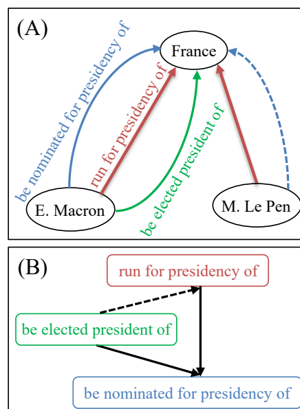
Figure 1: A link prediction knowledge graph (A) and an entailment graph (B) for entities of types politician, country . The solid lines are discovered correctly, but the dashed ones are missing. However, evidence from the link prediction model can be used to add the missing entailment rule in the entailment graph (B). Similarly, the entailment graph can be used to add the missing link in the knowledge graph (A).
