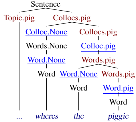
Figure 6: Sample parse generated by the collocation adaptor grammar. The adapted nonterminals \text{Colloc}_t and \text{Word}_t are shown underlined; the subtrees they dominate are “cached” by the adaptor grammar. The prefix (not shown here) is parsed exactly as in the Unigram PCFG.
