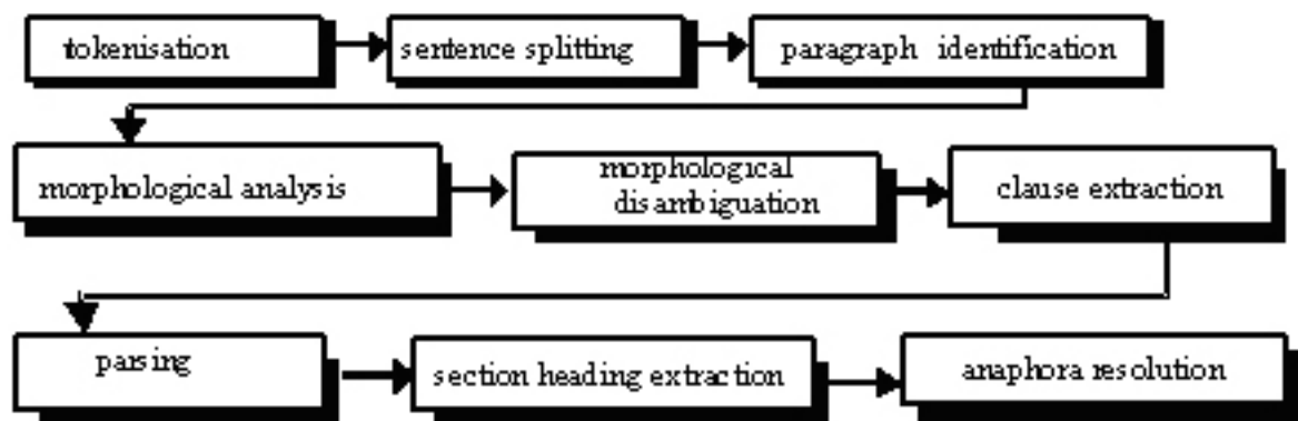
Figure 1: General architecture of LINGUA
