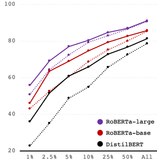
Figure 3: Three-run averages of F1 scores for tabular evidence extraction comparing the baseline model (TagOp), represented by dotted lines, to the tabular graph model (GEE), represented by solid lines. We trained the models with 1% to 100% of the training data (horizontal axis).
