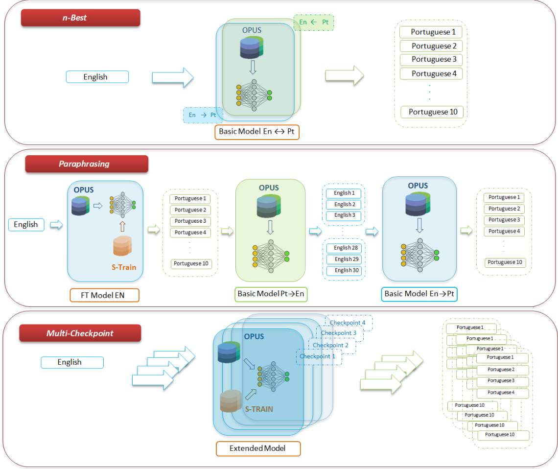
Figure 2: An illustration of our proposed models and methods: (a) n -Best prediction method with n = 10 resulting in the \text{En} \rightarrow \text{Pt} basic model; (b) paraphrasing method with n = 10 and n' = 3 used in the \text{En} \rightarrow \text{Pt} fine-tuning and the \text{En} \leftrightarrow \text{Pt} basic models, (c) multi-checkpoint method used with n = 10 and m = 4 for the \text{En} \rightarrow \text{Pt} extended model.
