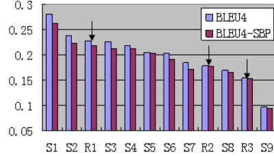
Figure 3. C2E News Translation Results.
