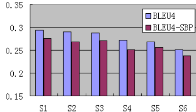
Figure 4. C2E System Combination Results.
